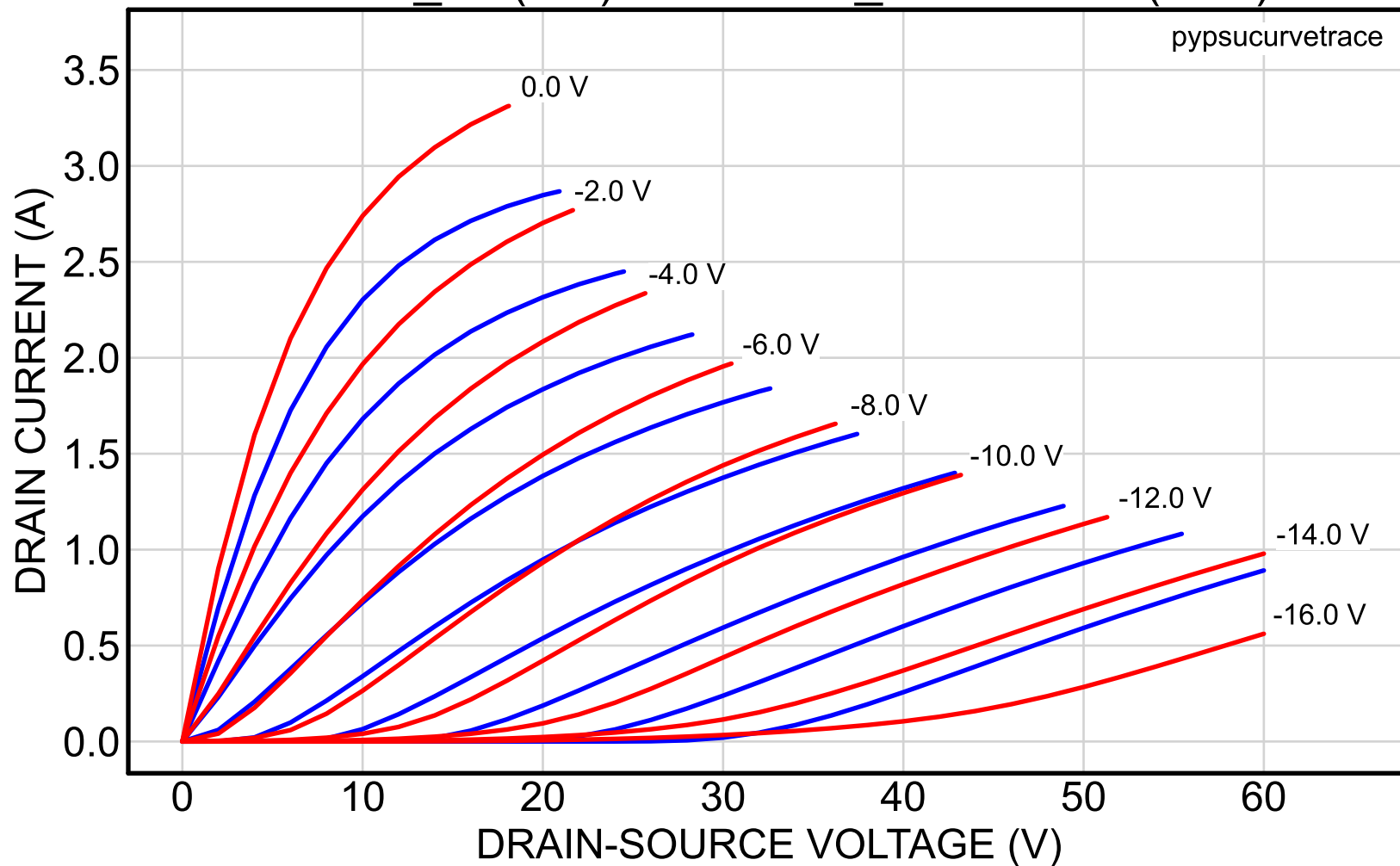
2SK82_35 (red) vs. 2SK82_40reserved (blue)
