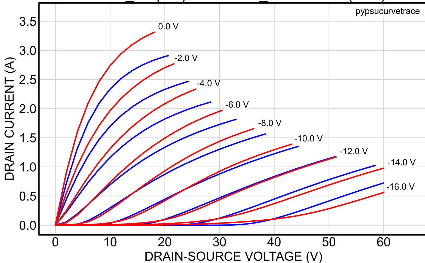
2SK82_35 (red) vs. 2SK82_56reserved (blue)
