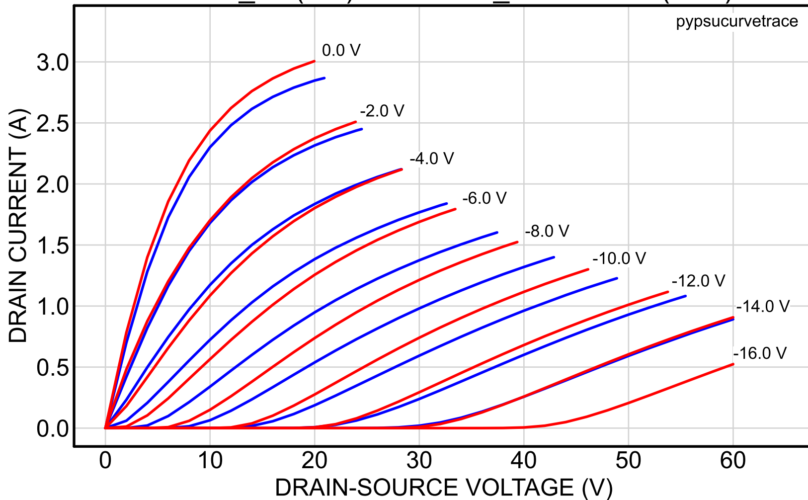
2SK82_36 (red) vs. 2SK82_40reserved (blue)
