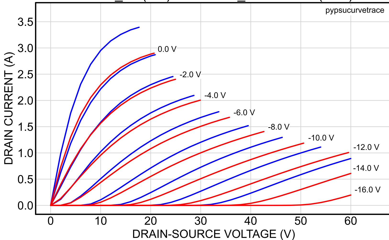
2SK82_38 (red) vs. 2SK82_39reserved (blue)
