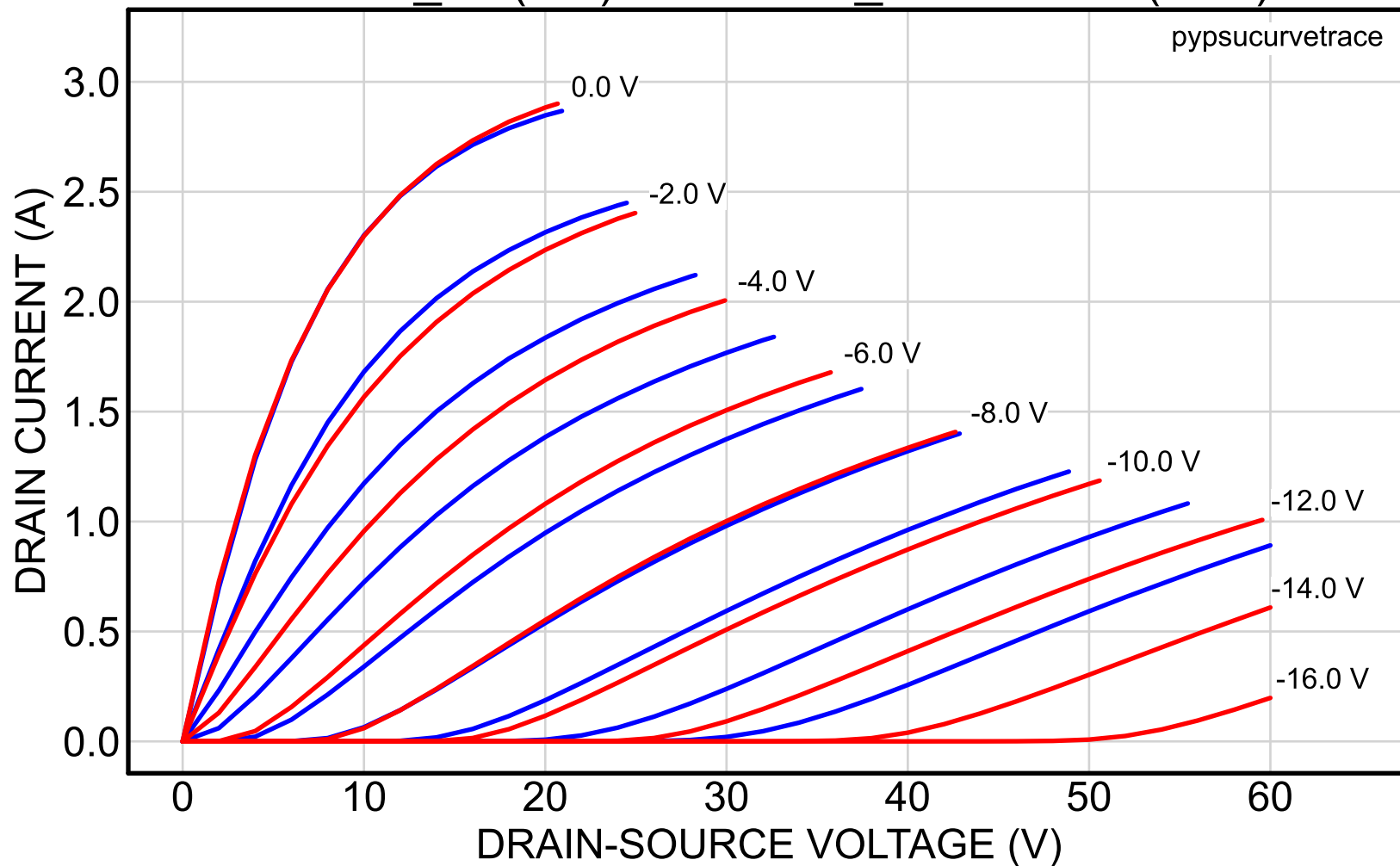
2SK82_38 (red) vs. 2SK82_40reserved (blue)
