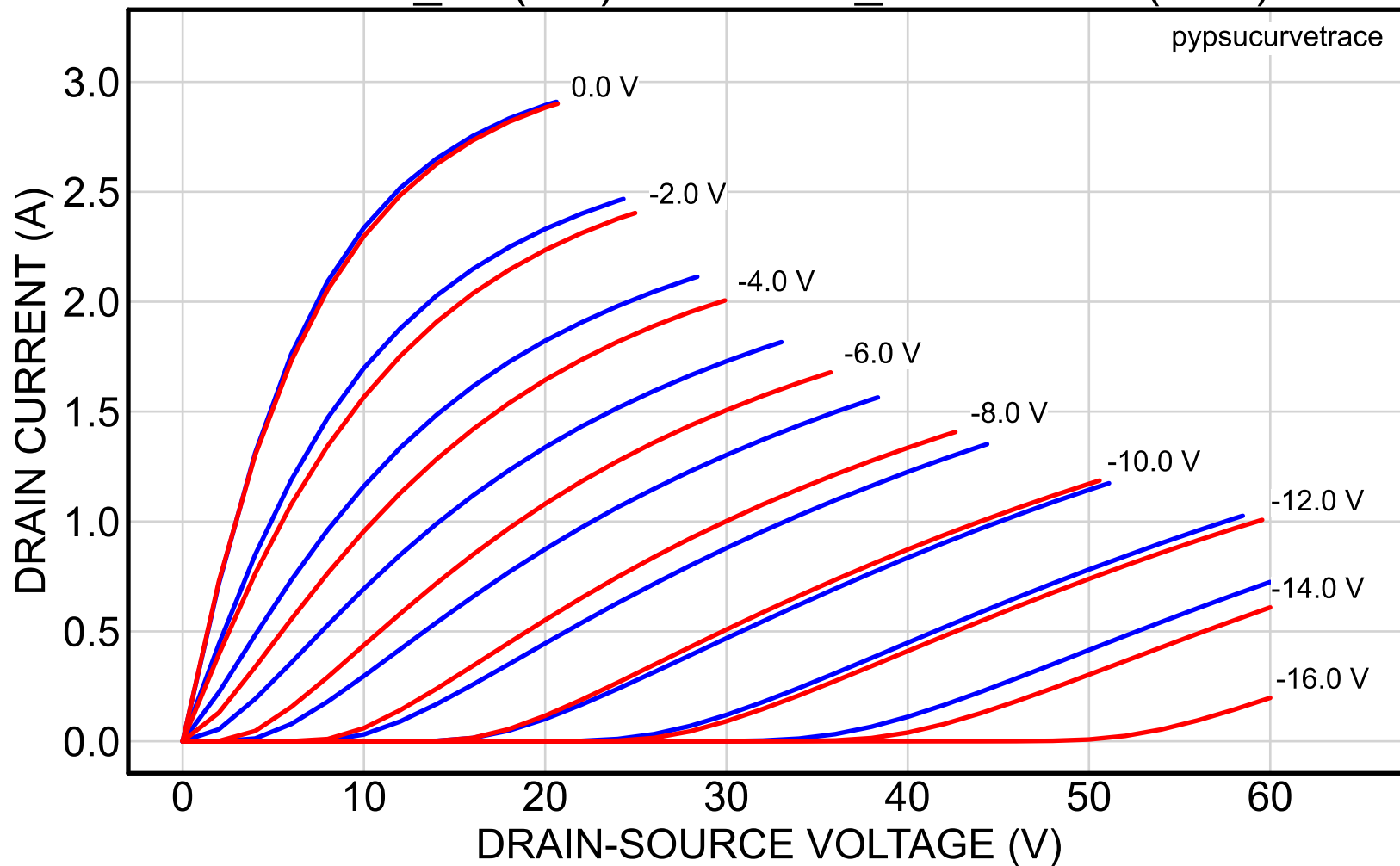
2SK82_38 (red) vs. 2SK82_56reserved (blue)
