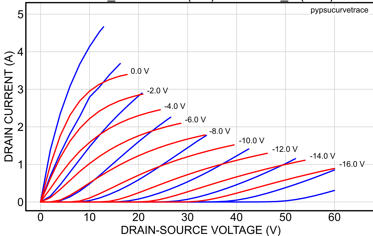
2SK82_39reserved (red) vs. 2SK82_3 (blue)
