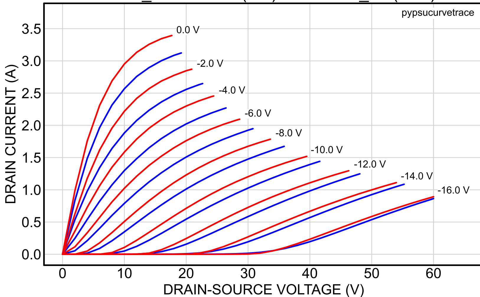
2SK82_39reserved (red) vs. 2SK82_41 (blue)
