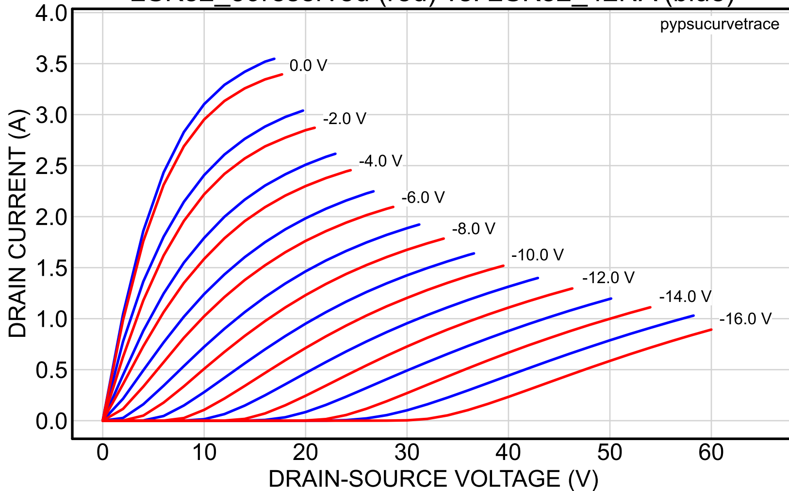
2SK82_39reserved (red) vs. 2SK82_42NA (blue)
