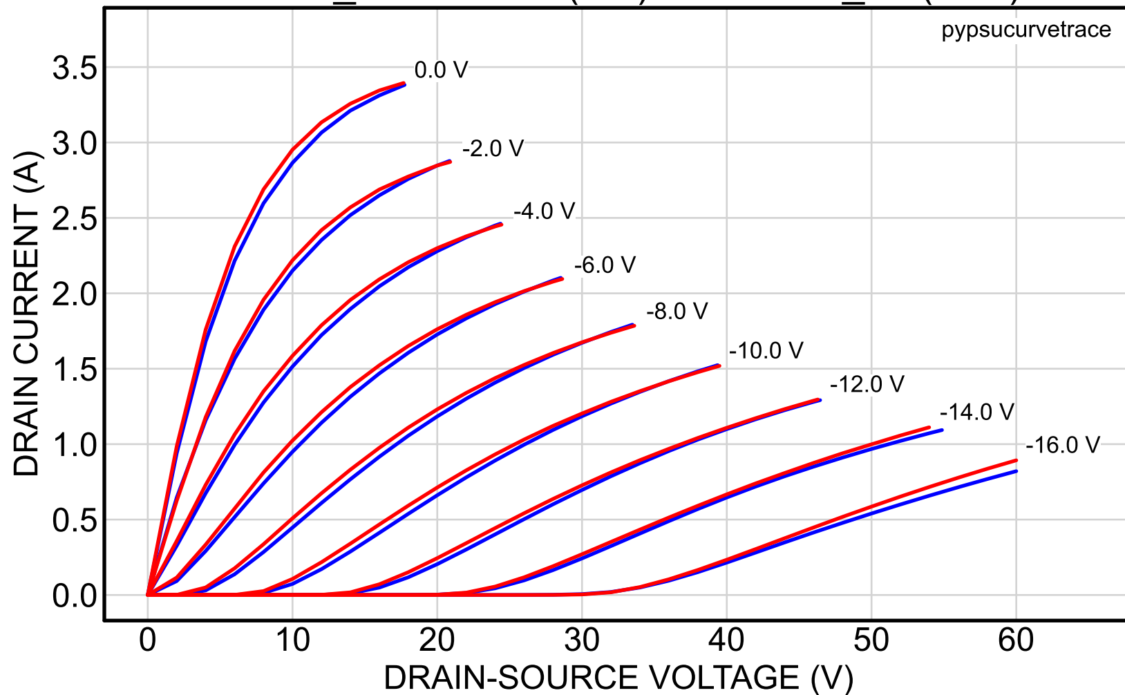
2SK82_39reserved (red) vs. 2SK82_43 (blue)
