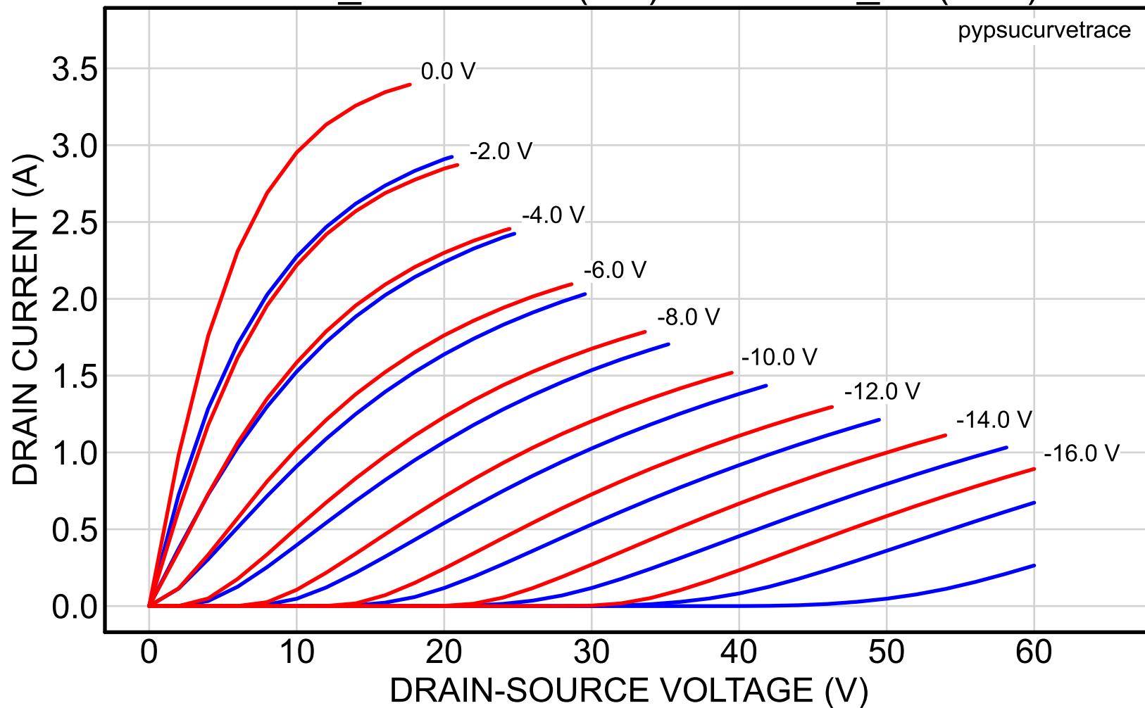
2SK82_39reserved (red) vs. 2SK82_44 (blue)
