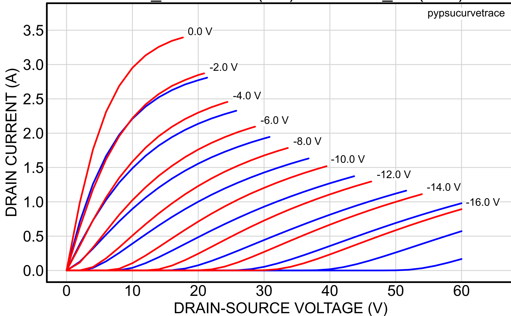
2SK82_39reserved (red) vs. 2SK82_45 (blue)
