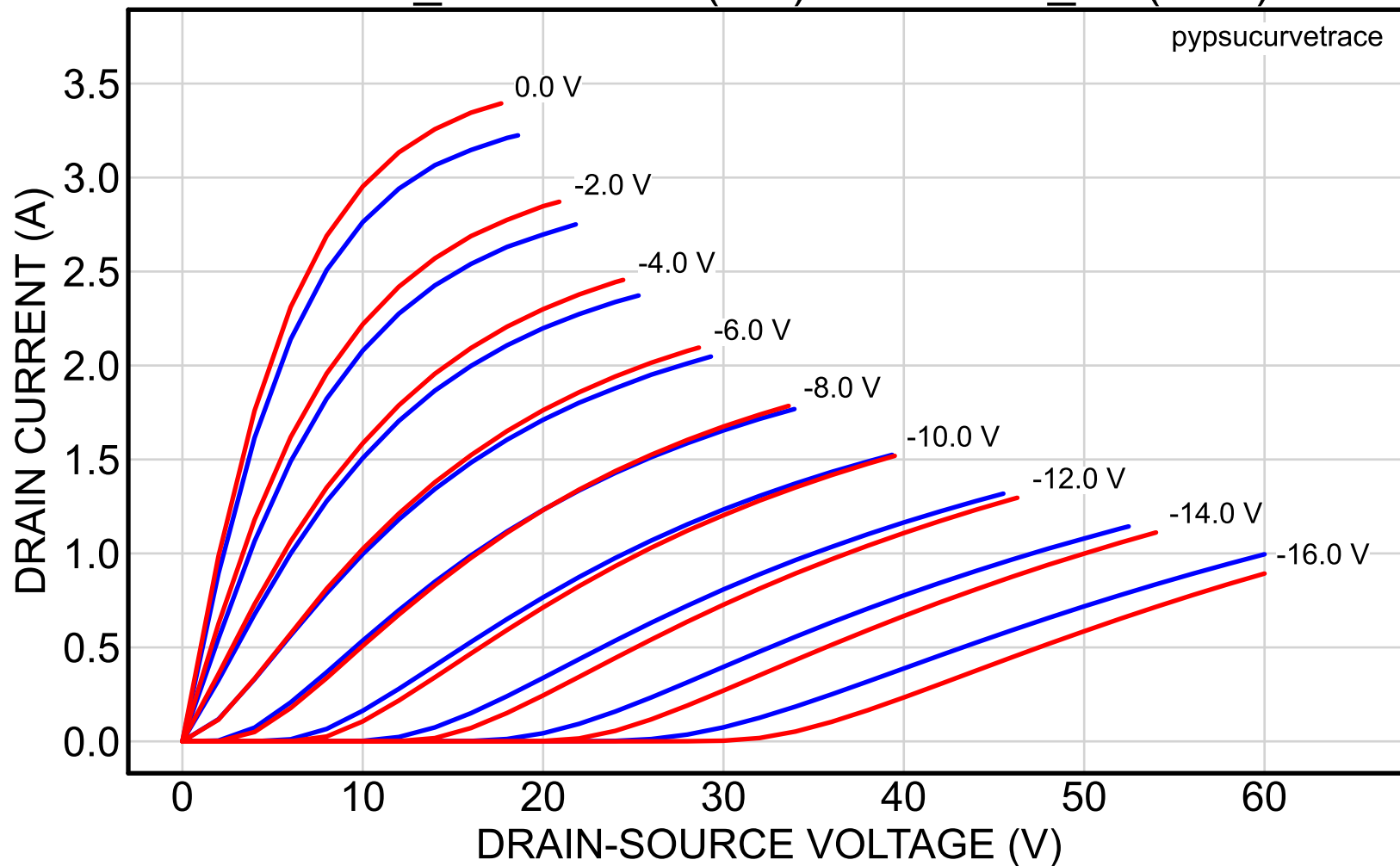
2SK82_39reserved (red) vs. 2SK82_46 (blue)
