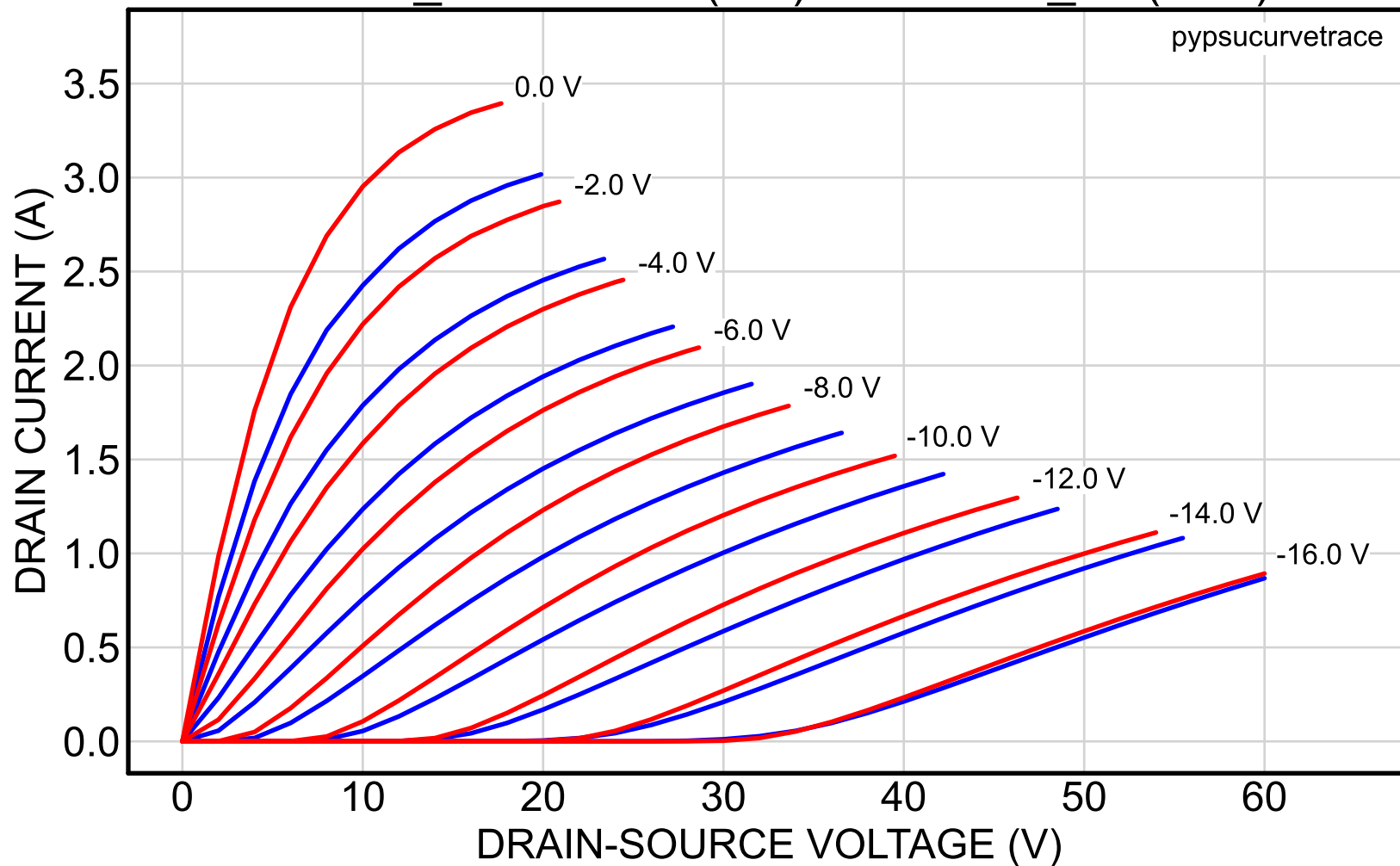
2SK82_39reserved (red) vs. 2SK82_47 (blue)
