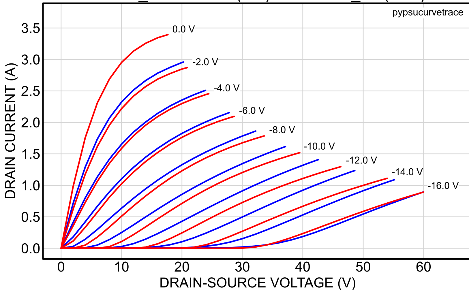
2SK82_39reserved (red) vs. 2SK82_48 (blue)
