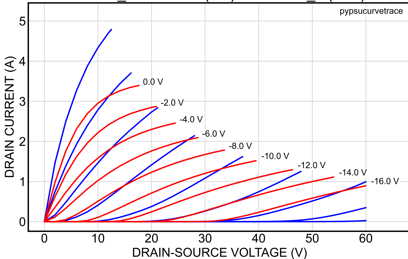
2SK82_39reserved (red) vs. 2SK82_4 (blue)
