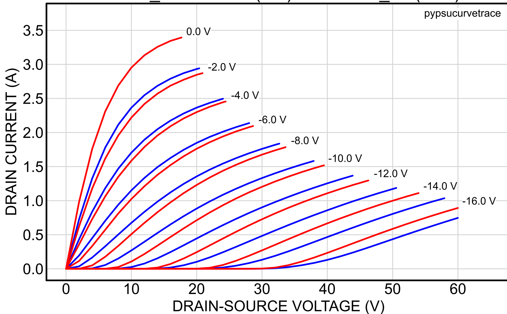
2SK82_39reserved (red) vs. 2SK82_50 (blue)
