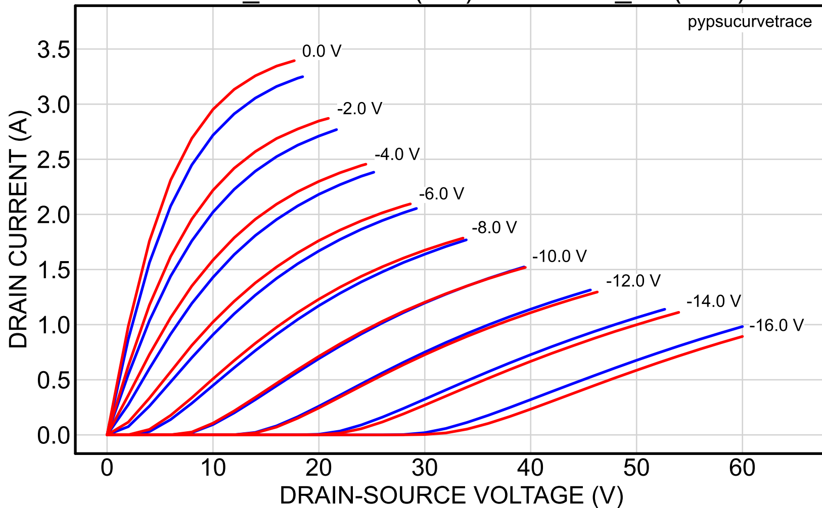
2SK82_39reserved (red) vs. 2SK82_53 (blue)
