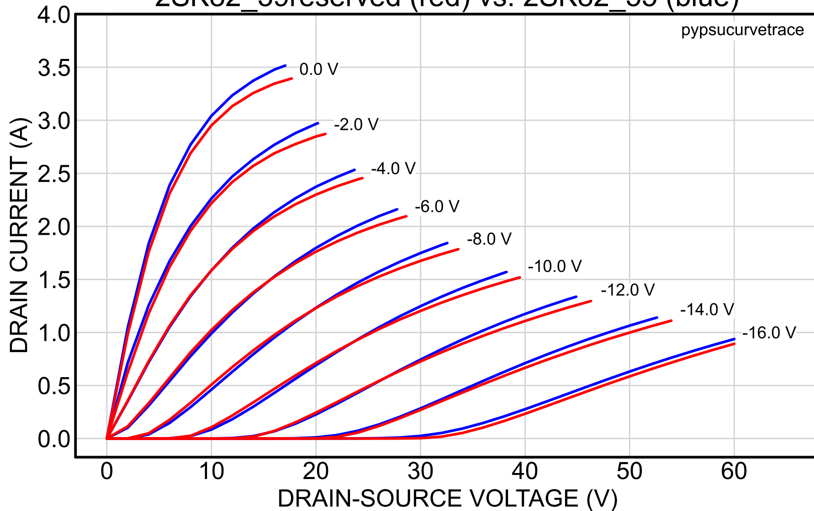
2SK82_39reserved (red) vs. 2SK82_55 (blue)
