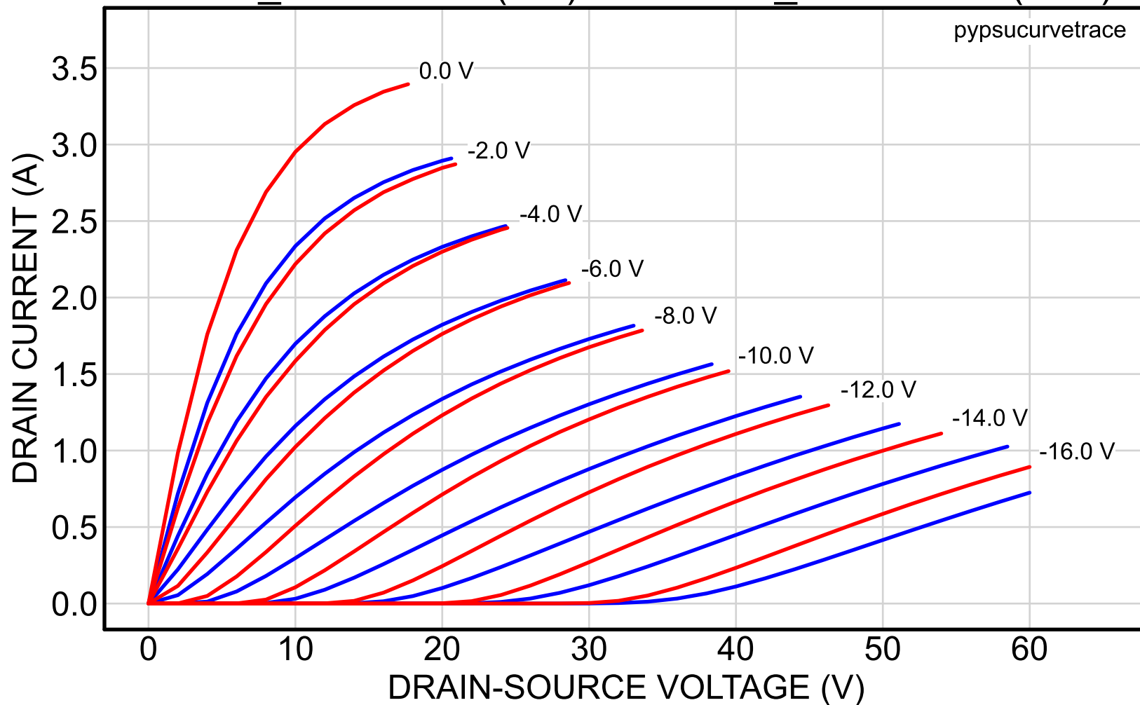
2SK82_39reserved (red) vs. 2SK82_56reserved (blue)
