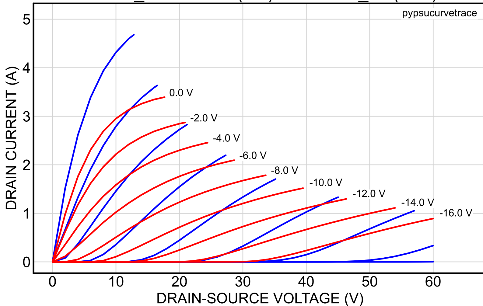
2SK82_39reserved (red) vs. 2SK82_57 (blue)
