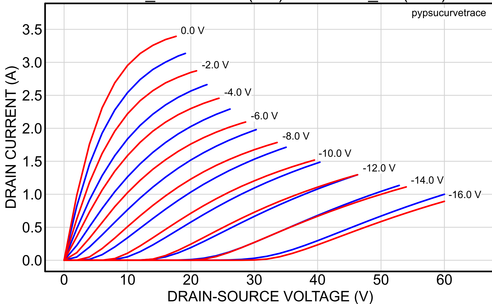
2SK82_39reserved (red) vs. 2SK82_59 (blue)
