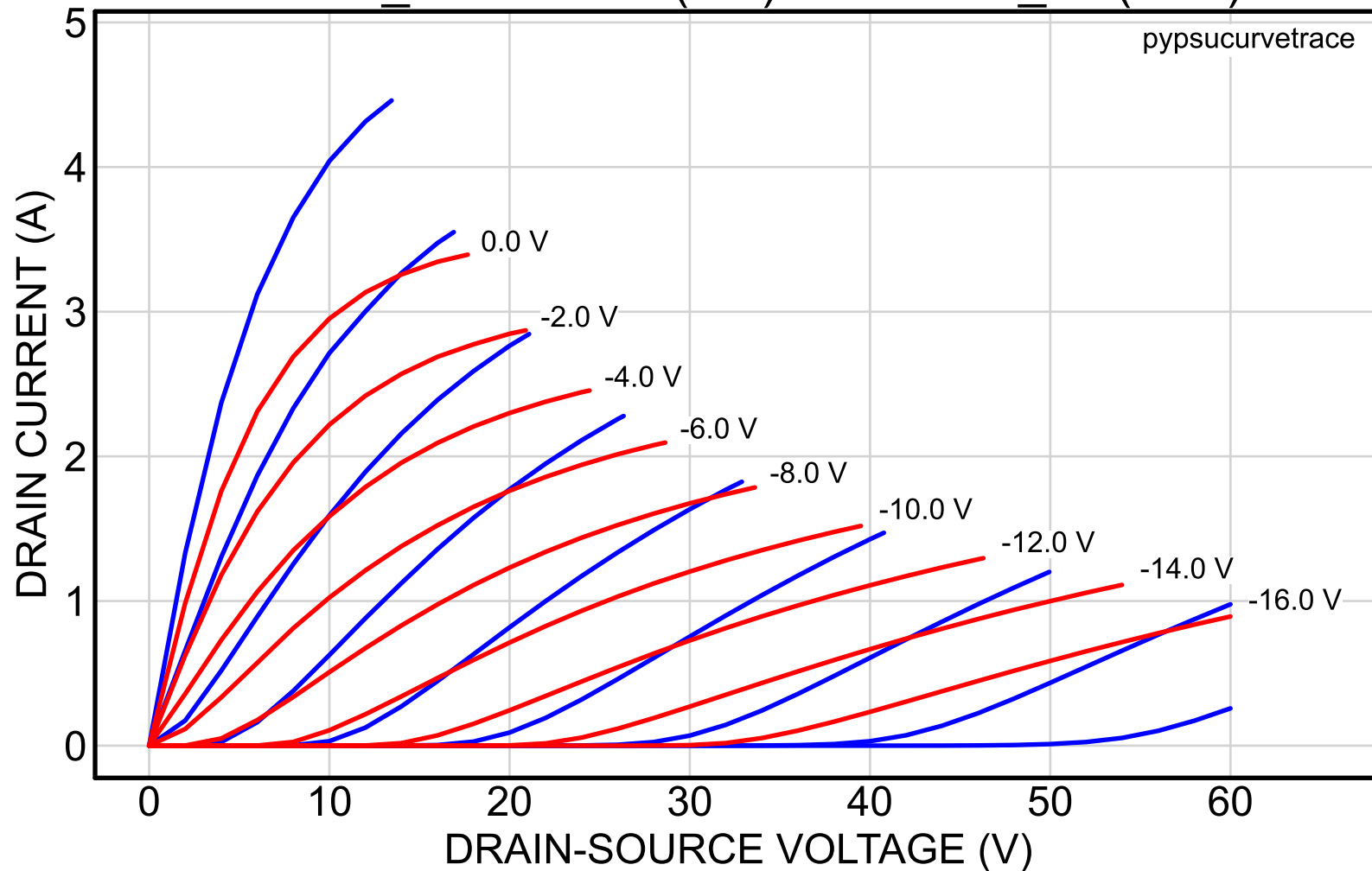
2SK82_39reserved (red) vs. 2SK82_60 (blue)
