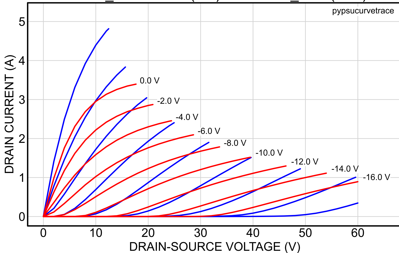
2SK82_39reserved (red) vs. 2SK82_6NA (blue)
