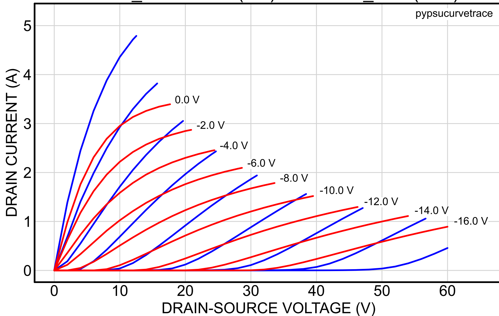
2SK82_39reserved (red) vs. 2SK82_8NA (blue)
