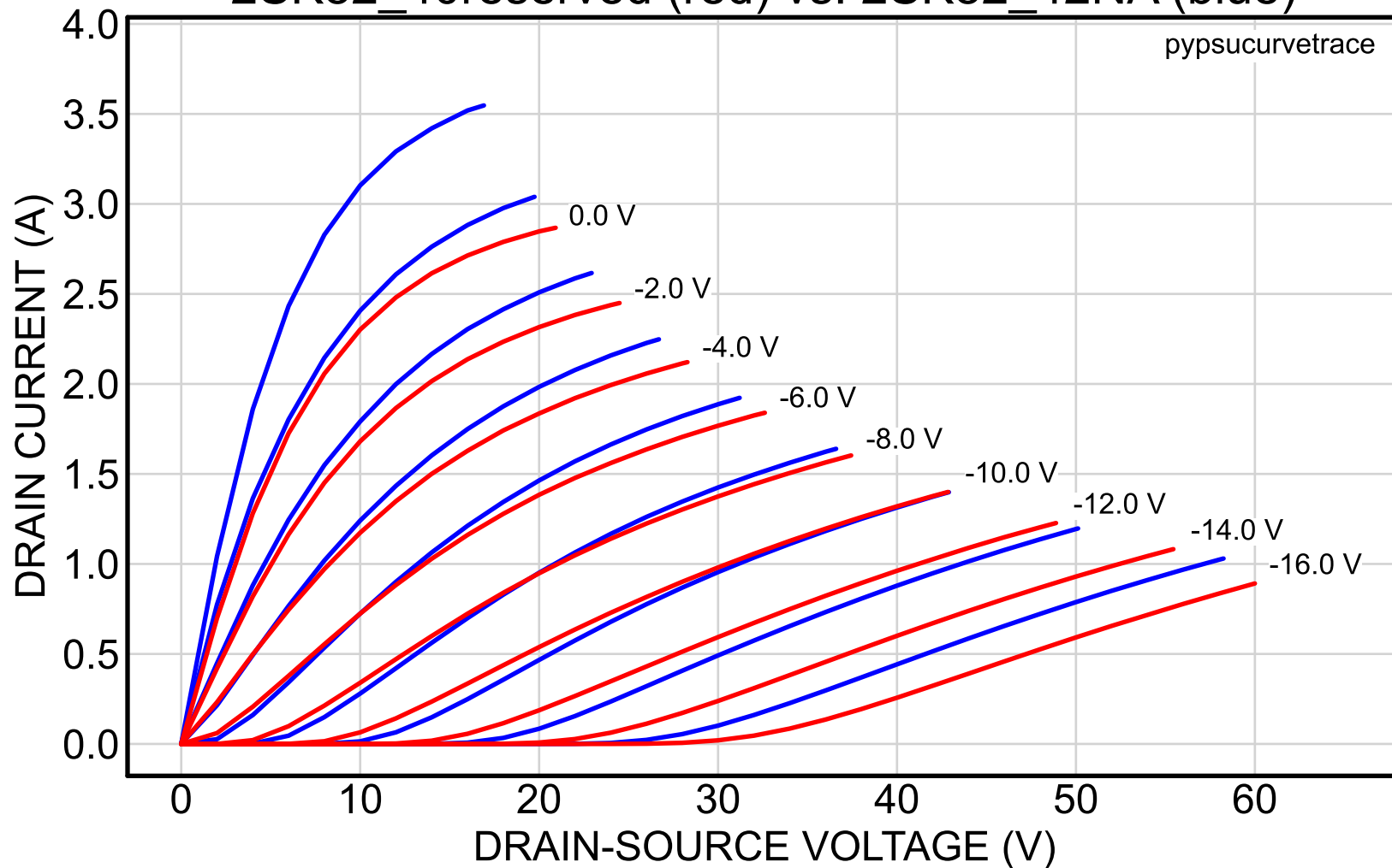
2SK82_40reserved (red) vs. 2SK82_42NA (blue)
