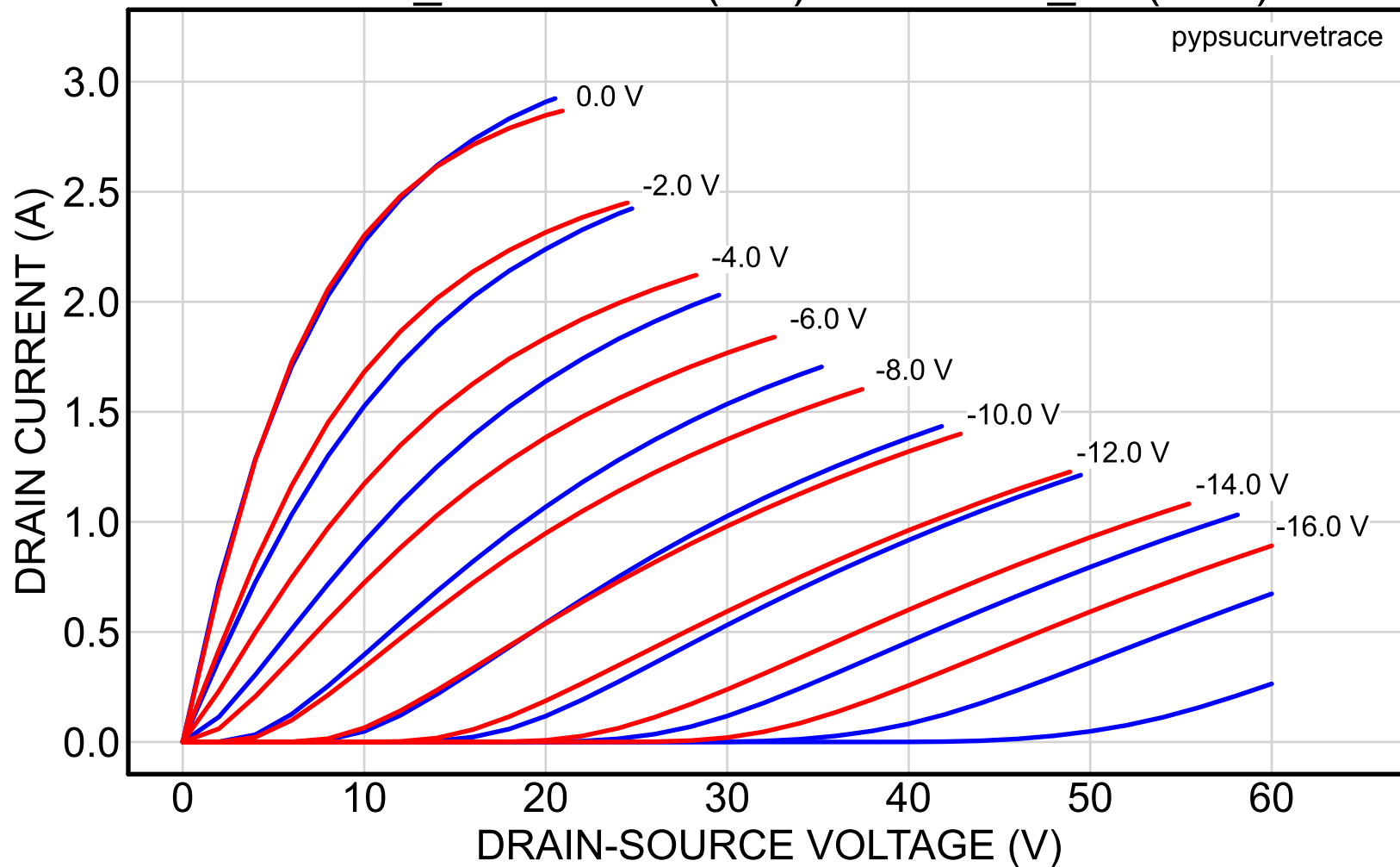
2SK82_40reserved (red) vs. 2SK82_44 (blue)
