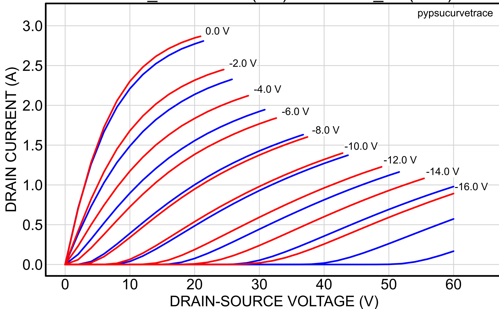
2SK82_40reserved (red) vs. 2SK82_45 (blue)
