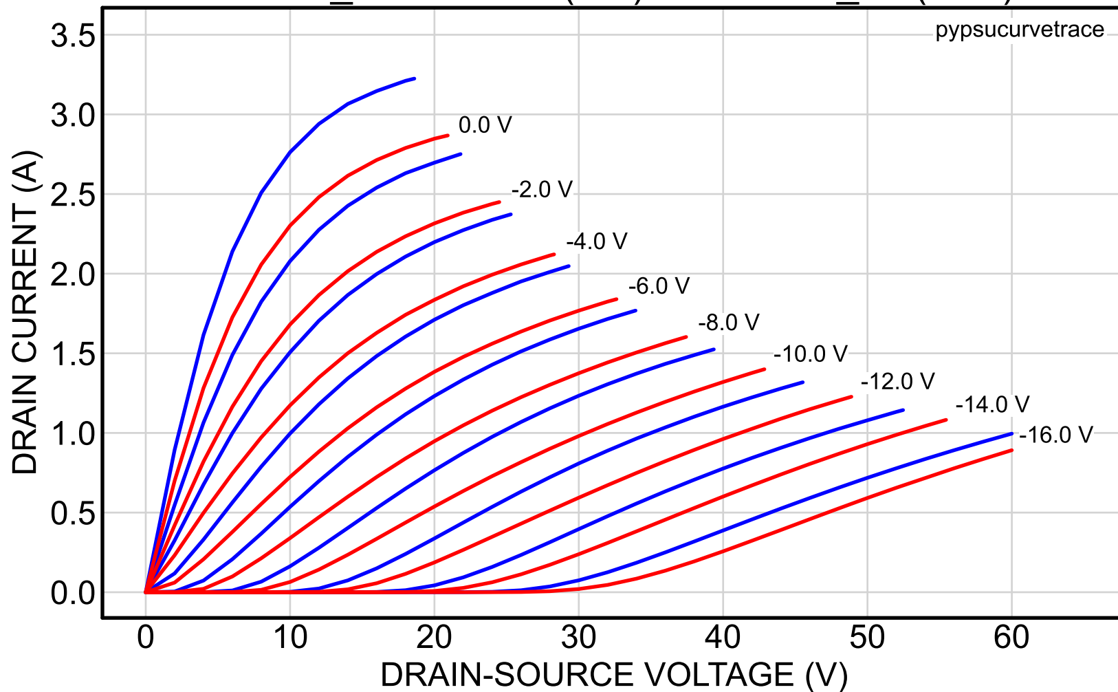
2SK82_40reserved (red) vs. 2SK82_46 (blue)
