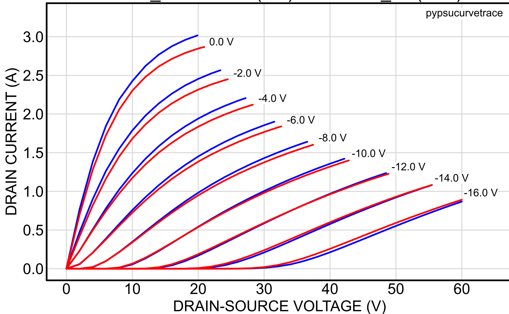
2SK82_40reserved (red) vs. 2SK82_47 (blue)
