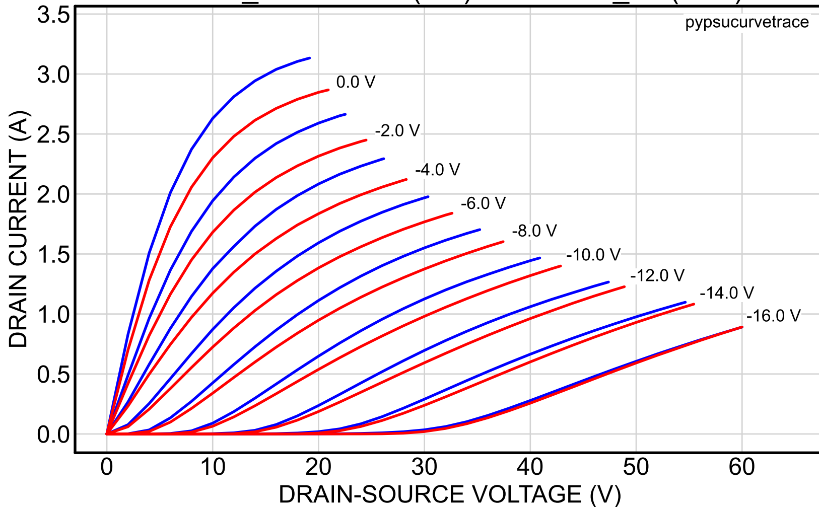
2SK82_40reserved (red) vs. 2SK82_49 (blue)
