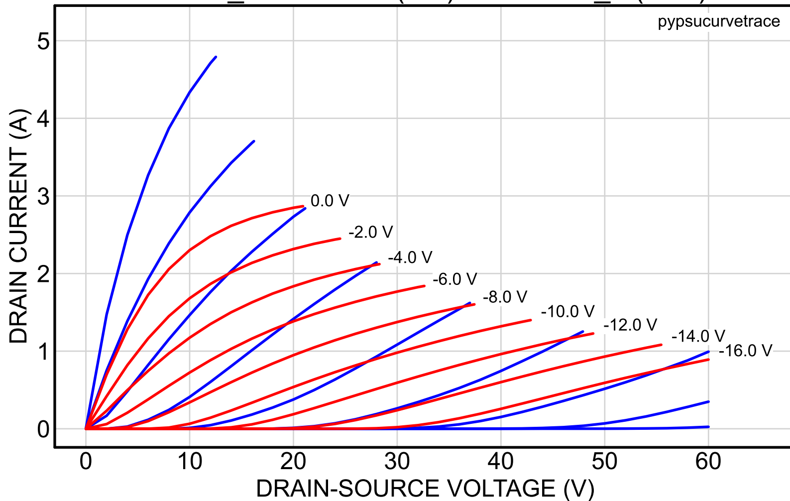
2SK82_40reserved (red) vs. 2SK82_4 (blue)
