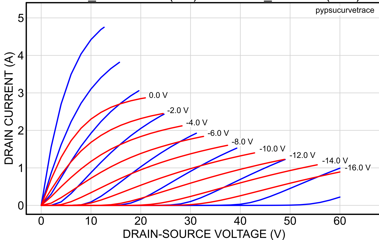
2SK82_40reserved (red) vs. 2SK82_51NAbb (blue)
