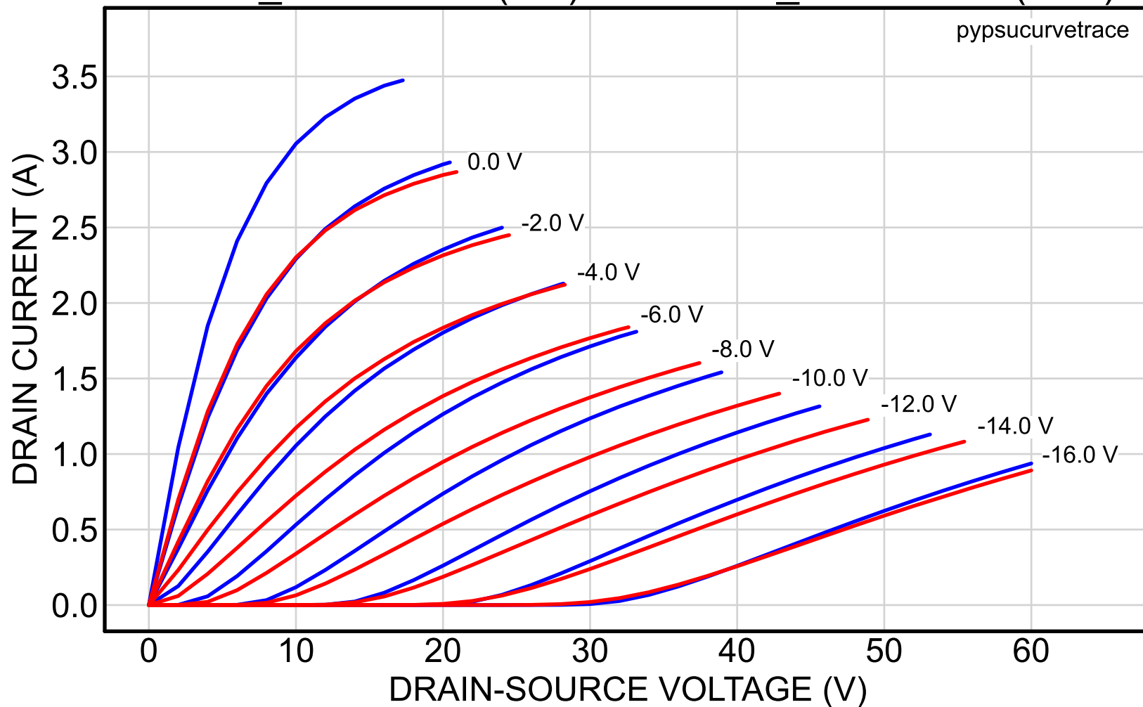
2SK82_40reserved (red) vs. 2SK82_52reserved (blue)
