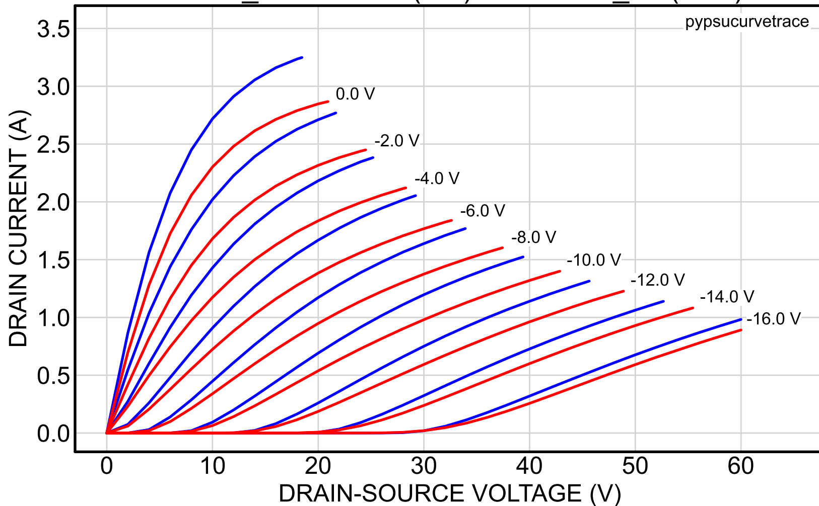
2SK82_40reserved (red) vs. 2SK82_53 (blue)
