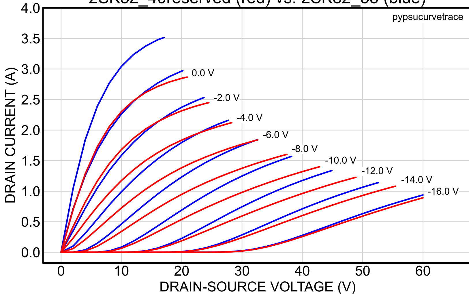
2SK82_40reserved (red) vs. 2SK82_55 (blue)
