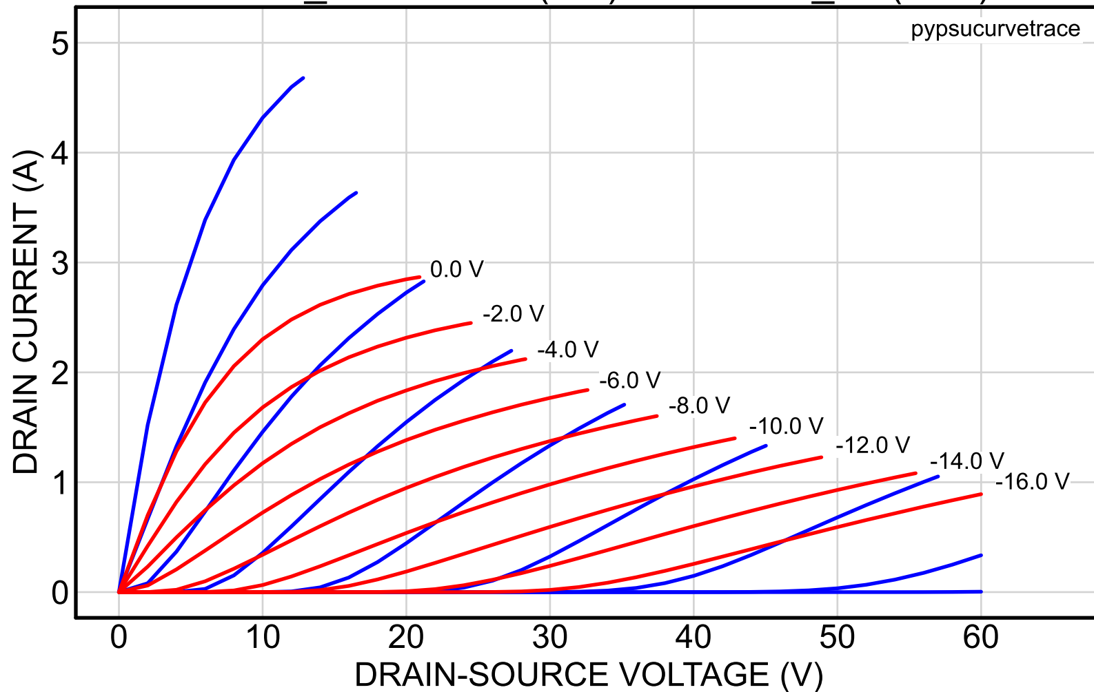
2SK82_40reserved (red) vs. 2SK82_57 (blue)
