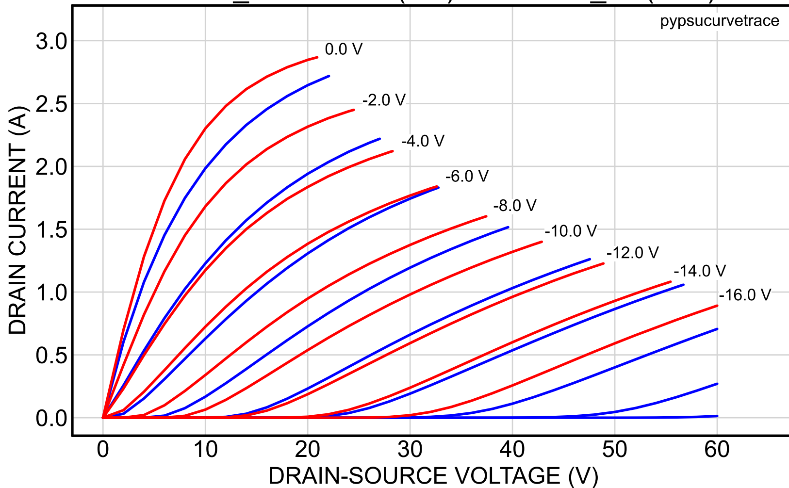
2SK82_40reserved (red) vs. 2SK82_58 (blue)
