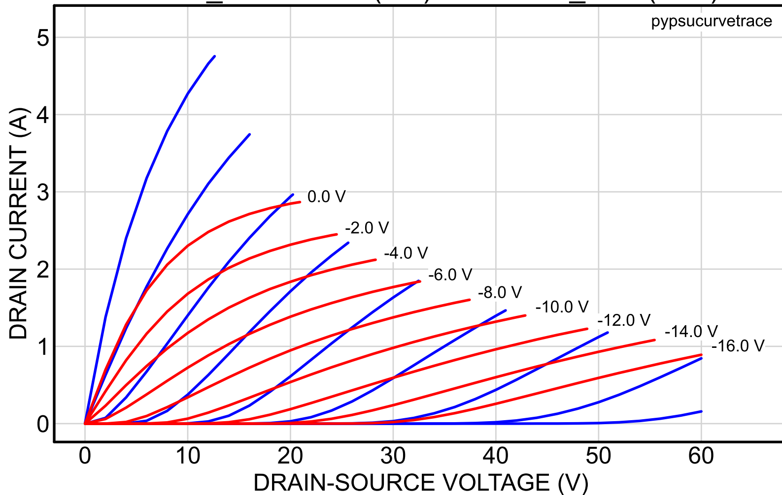
2SK82_40reserved (red) vs. 2SK82_5NA (blue)
