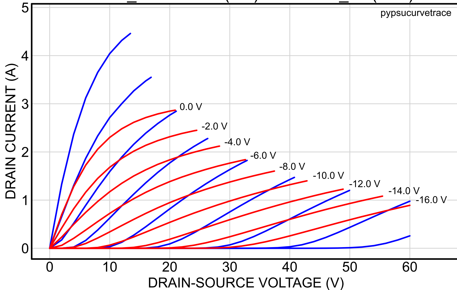
2SK82_40reserved (red) vs. 2SK82_60 (blue)
