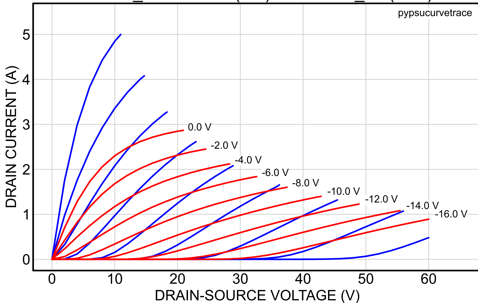
2SK82_40reserved (red) vs. 2SK82_61 (blue)
