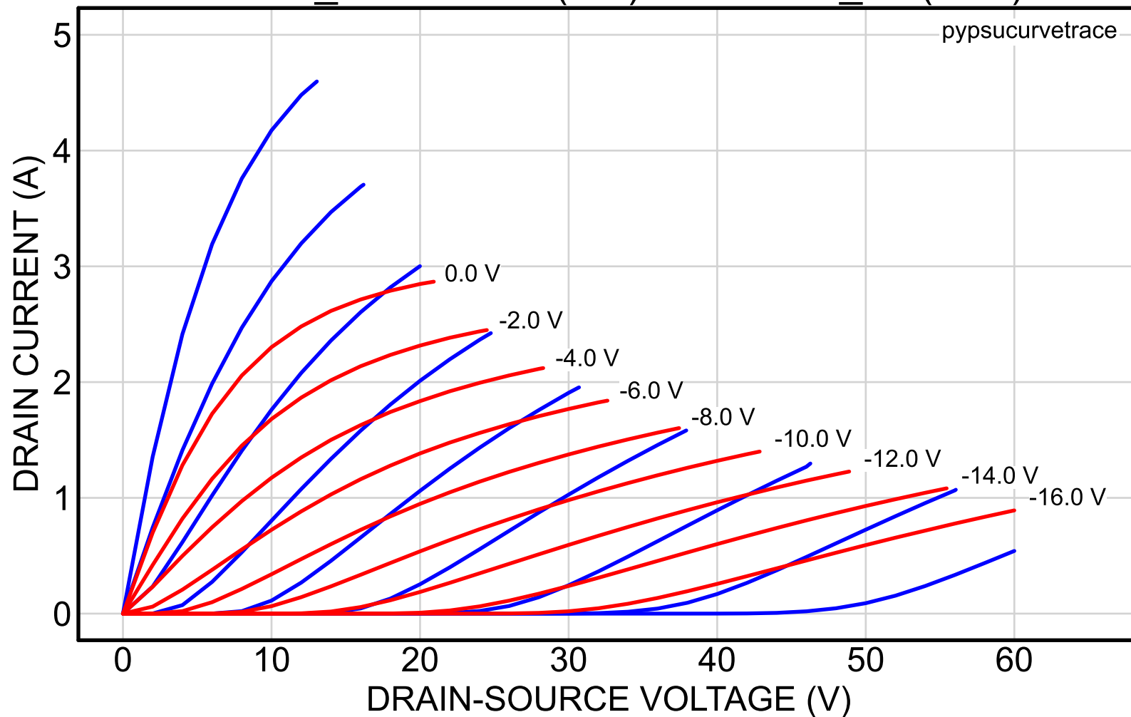
2SK82_40reserved (red) vs. 2SK82_62 (blue)
