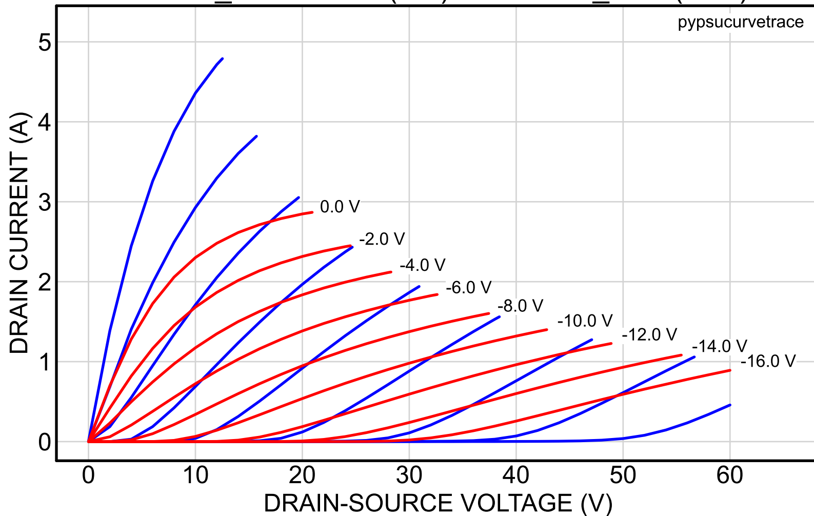
2SK82_40reserved (red) vs. 2SK82_8NA (blue)
