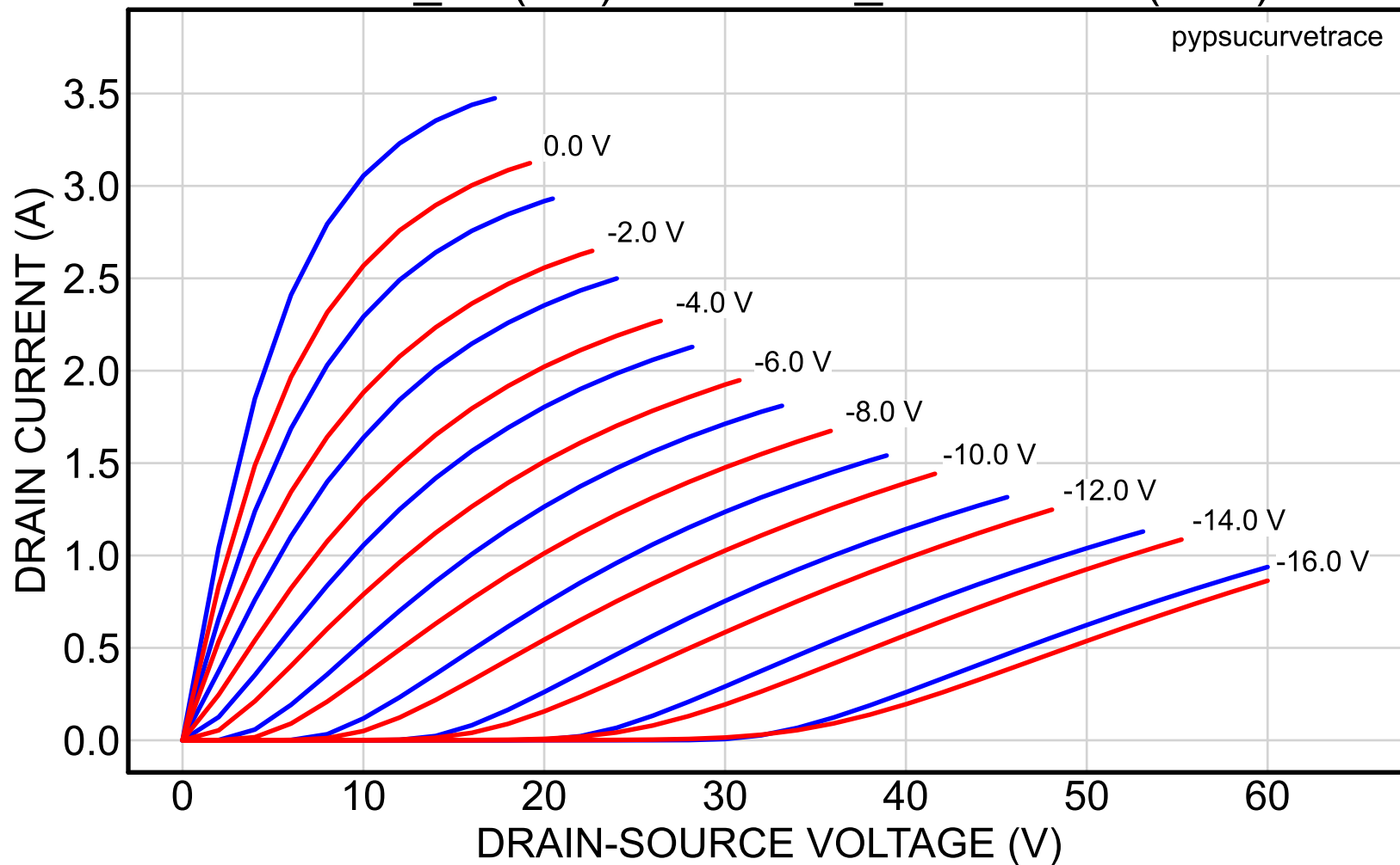
2SK82_41 (red) vs. 2SK82_52reserved (blue)
