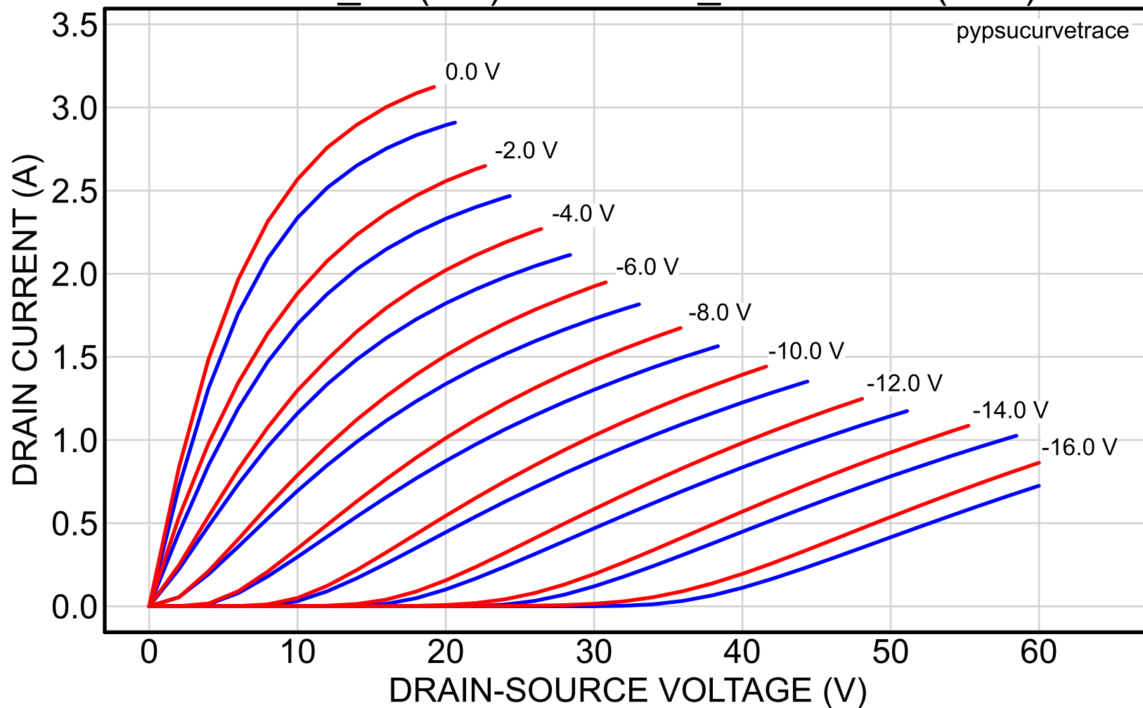
2SK82_41 (red) vs. 2SK82_56reserved (blue)
