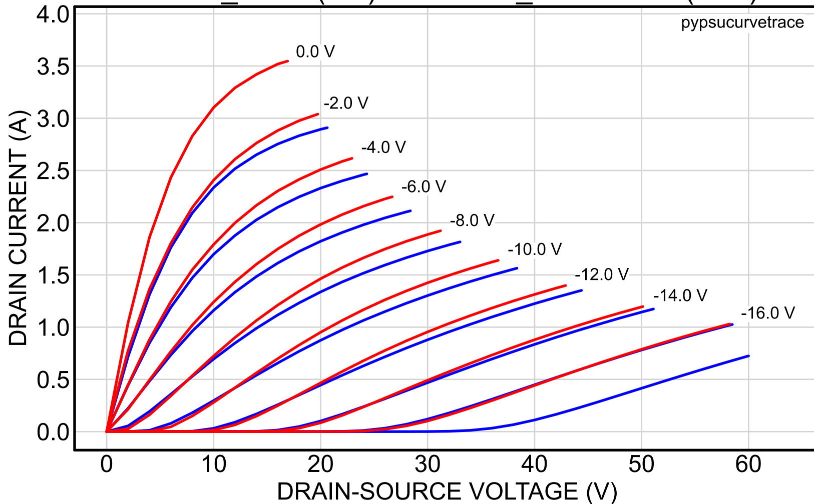
2SK82_42NA (red) vs. 2SK82_56reserved (blue)
