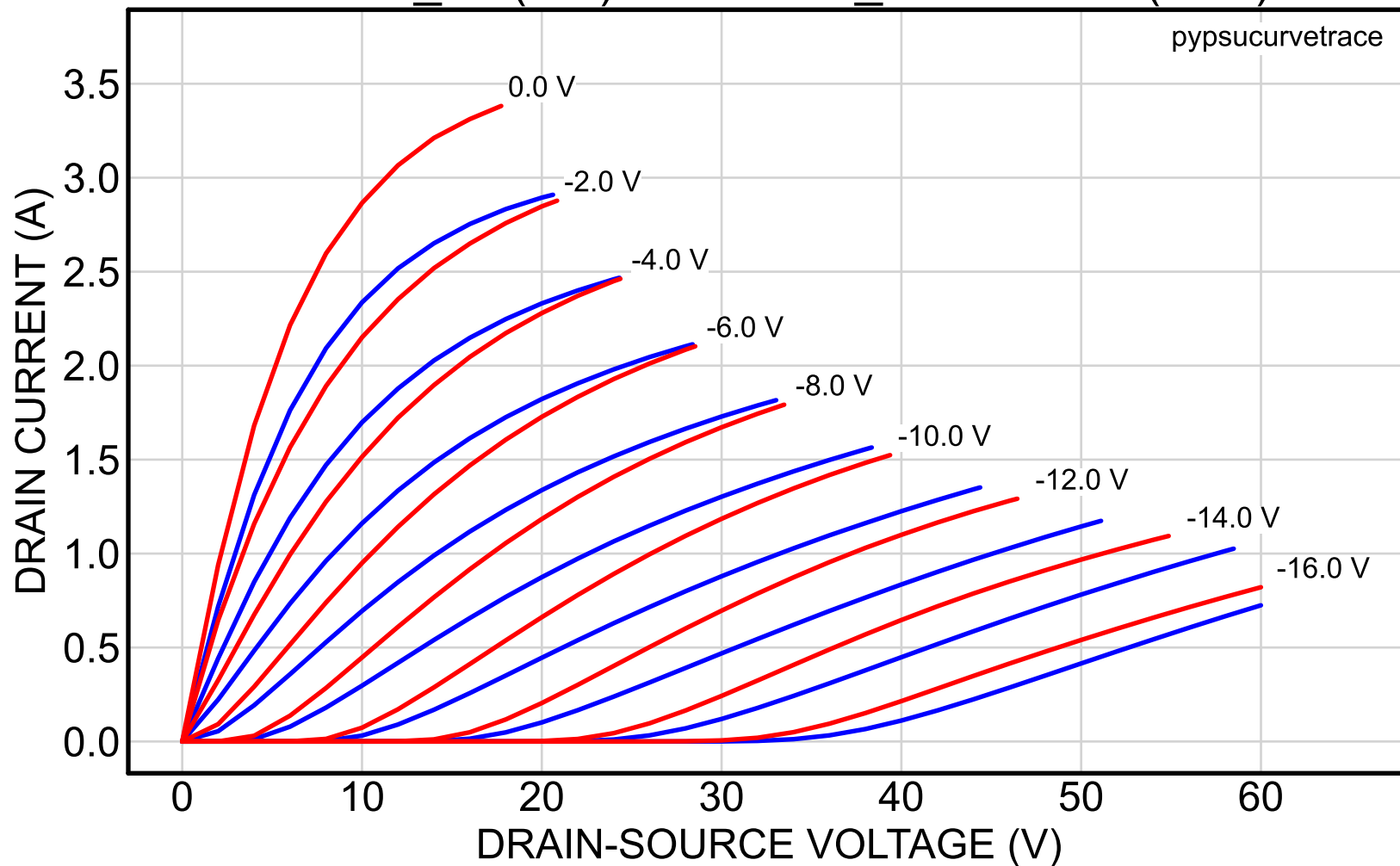
2SK82_43 (red) vs. 2SK82_56reserved (blue)
