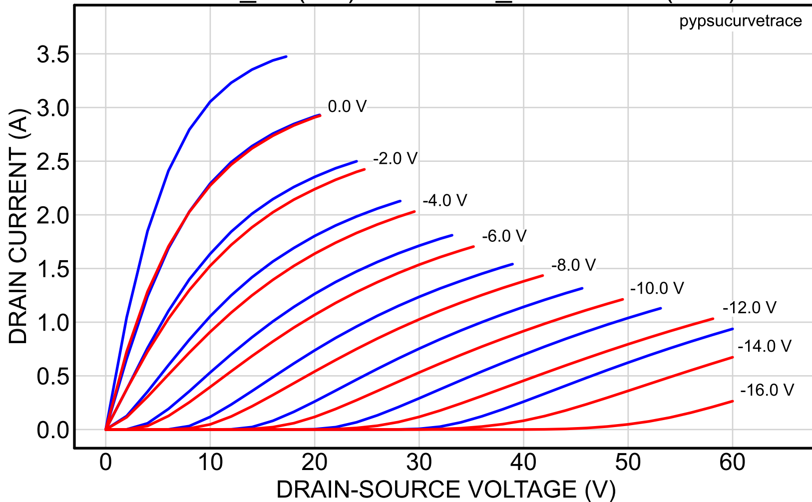
2SK82_44 (red) vs. 2SK82_52reserved (blue)
