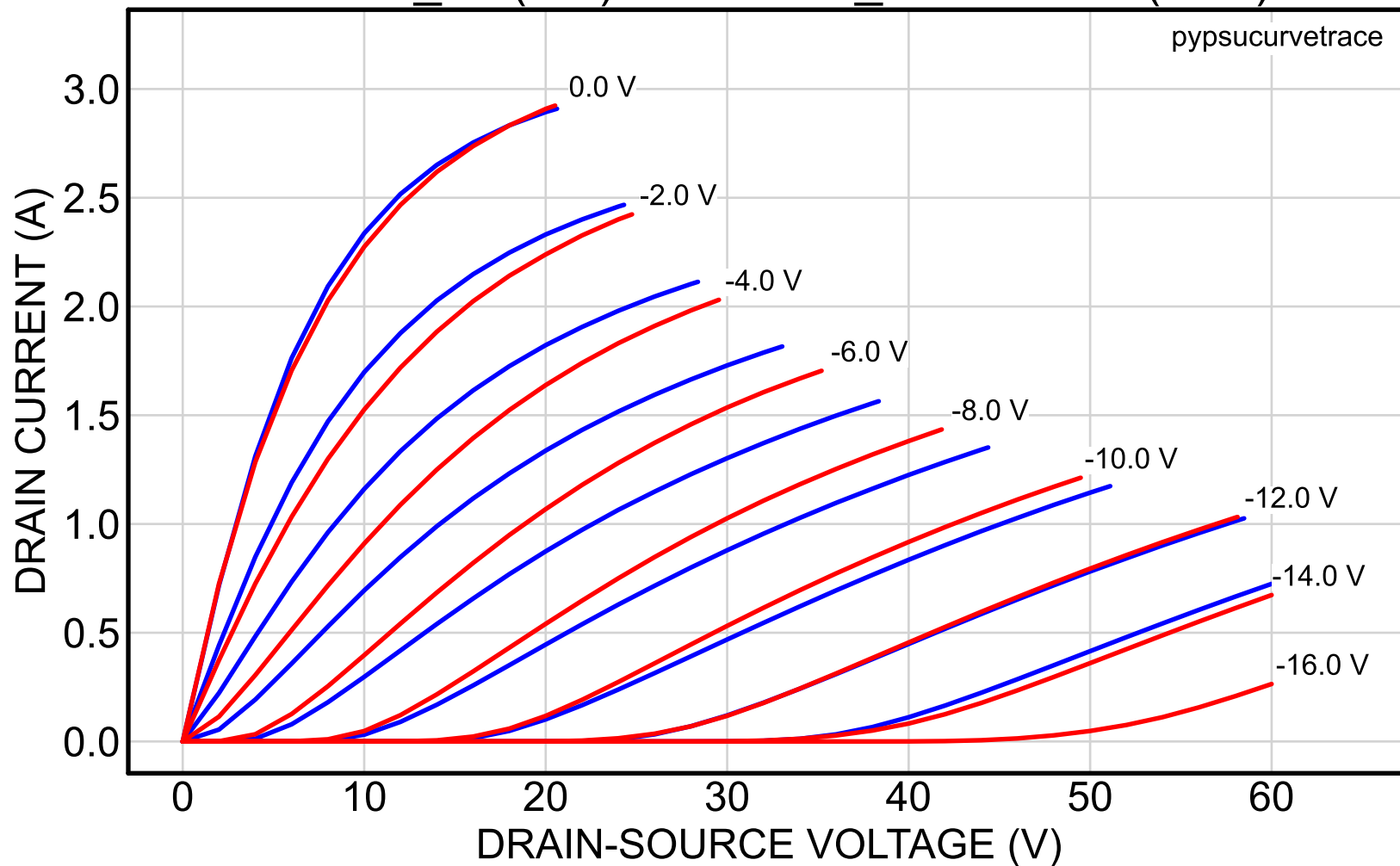
2SK82_44 (red) vs. 2SK82_56reserved (blue)
