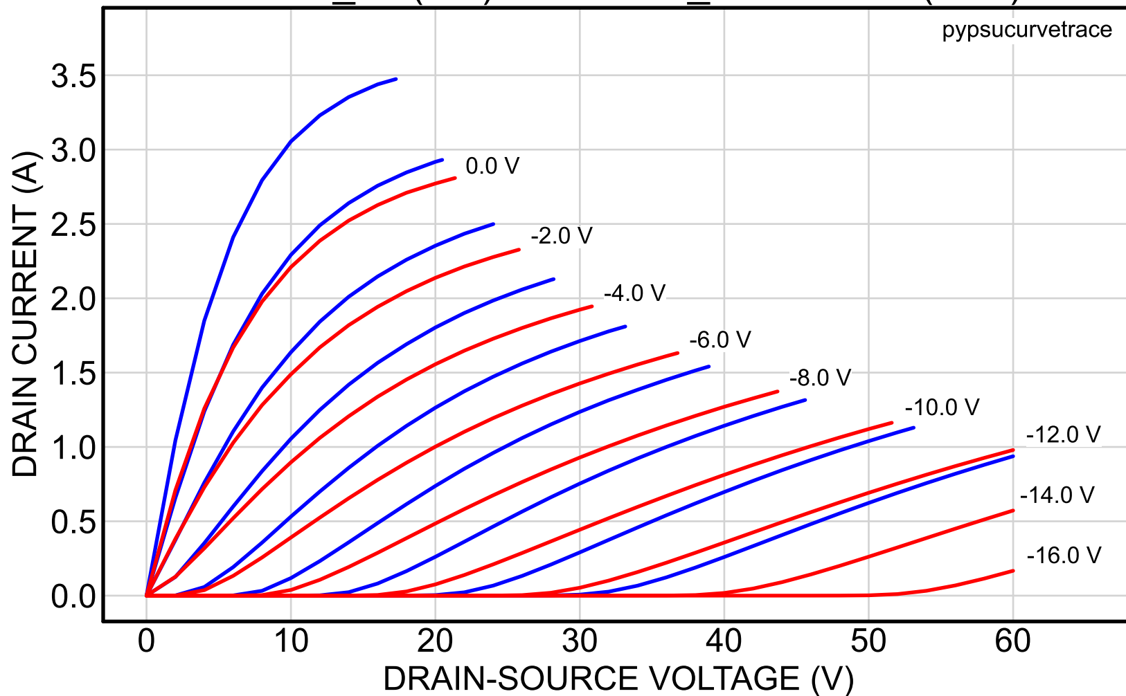
2SK82_45 (red) vs. 2SK82_52reserved (blue)
